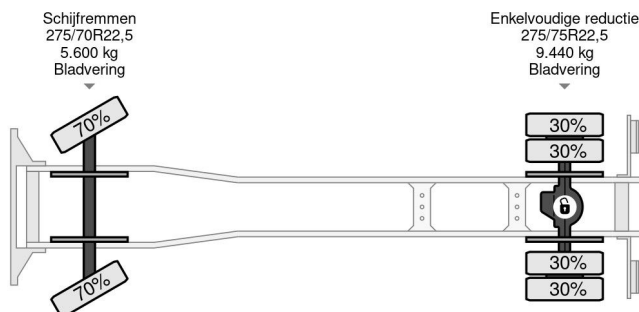
Renault Midlum 280 DXI FULL STEEL SUSPENSION 3... 4x2 Referentienummer: SN 58100390
