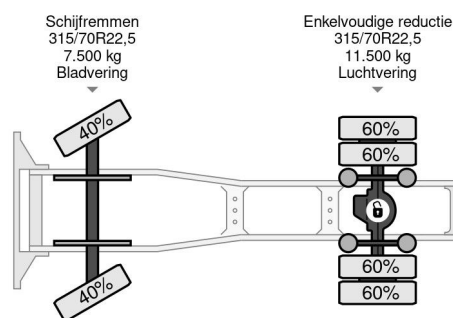
MAN 19.414 XT (F2000) (6-CILINDER HEADS / ZF16 ... 4x2
